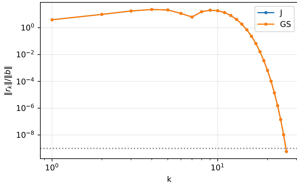
kahan, n = 30
